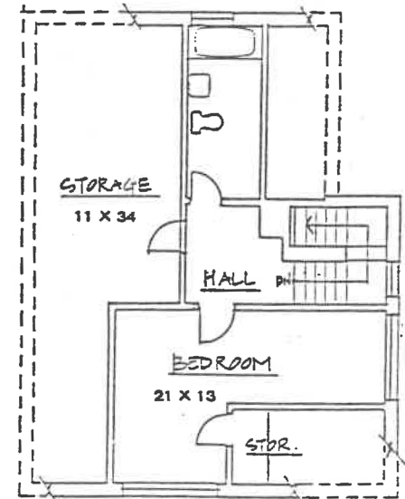
ATTIC PLAN
