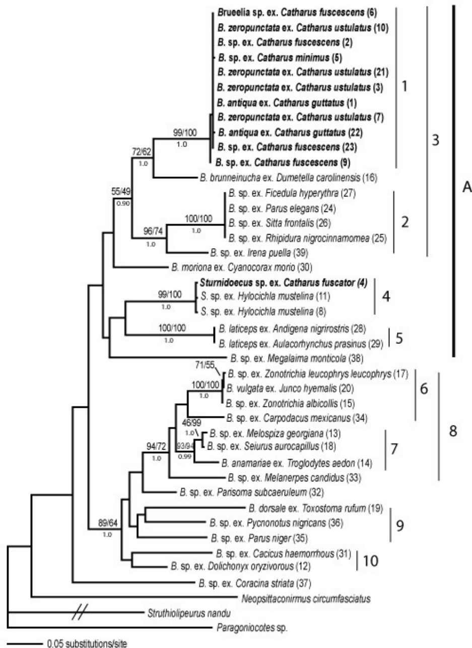
Figure 2: Molecular phylogeny of the genus Brueelia based on 385 bp of CO1 and 347 bp of EF1α. Maximum likelihood values are above the node (<50% support of 1000 bootstrap replicates), maximum parsimony values are beside them (<50% 1000 bootstrap replicate support), and Bayesian posterior probabilities are below the node (consensus of 5,000,000 samples trees < 0.90). The hash marks represent a shortening of the Struthiolipeurus nandu branch. Bold taxa are parasites from Catharus hosts.
