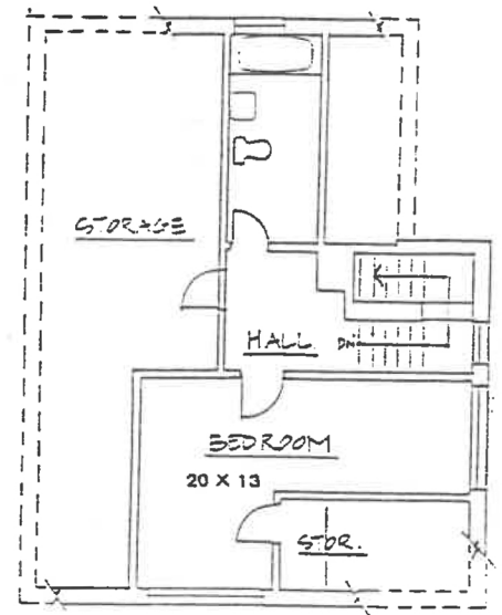
ATTIC PLAN
